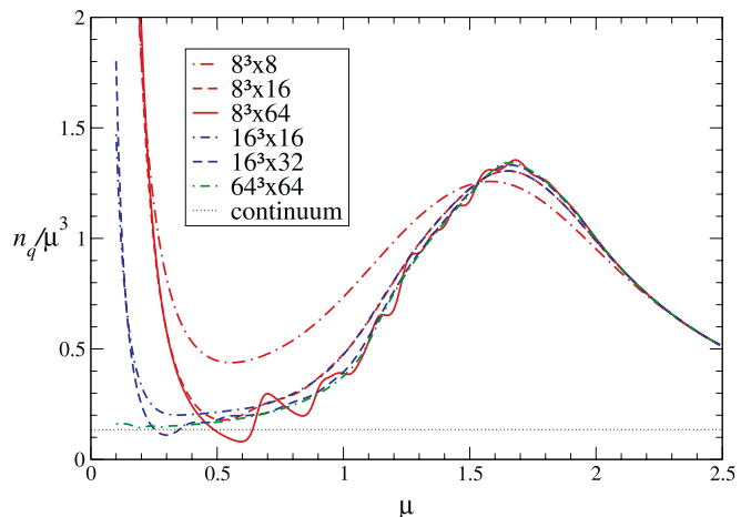
Fig. 4. n_{\text{SB}}^{\text{lat}}/\mu^3 for free massless Wilson fermions
