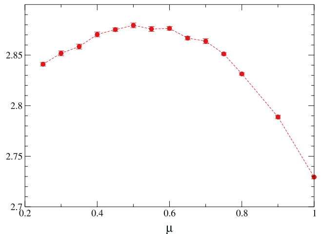
Fig. 8. Top: \kappa^{-1} \text{Tr}(1 - \langle\bar{\psi}\psi\rangle) , and bottom: 3\beta/N_c \text{Tr}(\square_t + \square_s) , as functions of \mu at j = 0.04
