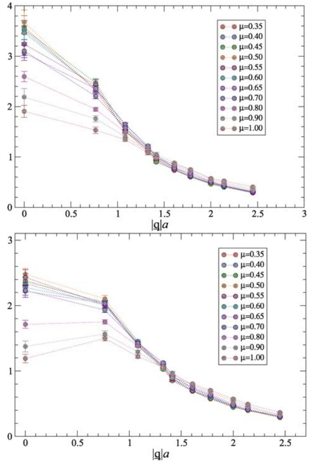
Fig. 17. Magnetic gluon propagator for q_0 = 0 (top) and aq_0 = 2 \sin \pi/16 (bottom) and diquark source j = 0.04 , as a function of spatial momentum |\mathbf{q}| for various values of the chemical potential
