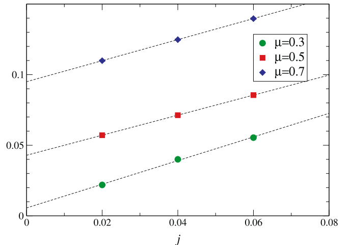
Fig. 11. Superfluid condensate \langle qq \rangle vs. j for various \mu
