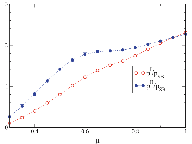
Fig. 6. Pressure versus \mu using two different integral methods
