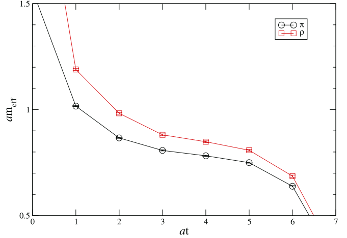
Fig. 1. Pi and rho effective masses for \mu = j = 0
