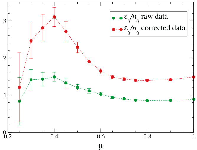
Fig. 20. The ratio \varepsilon_q/n_q vs. \mu , using both the raw data of Table 4, and rescaled by a factor n_{SB}^{\text{lat}}/\varepsilon_{SB}^{\text{lat}}
