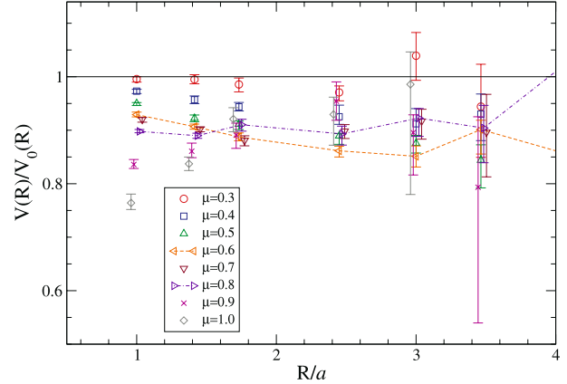
Fig. 13. The static quark potential for various values of the chemical potential \mu and diquark source j = 0.04 , divided the \mu = j = 0 potential shown in Fig. 2
