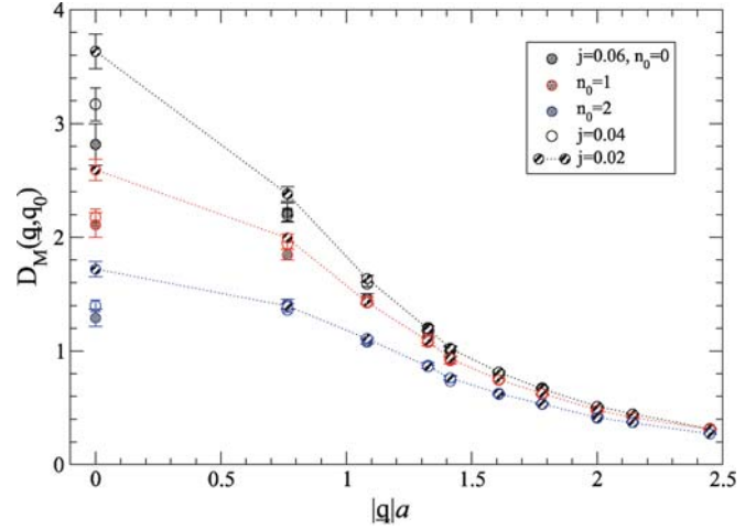
Fig. 19. Magnetic gluon propagator at \mu = 0.7 for various values of the diquark source j
