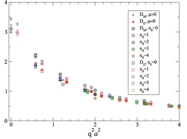
Fig. 16. Gluon propagator at \mu = 0.7, j = 0.04 , together with the \mu = j = 0 propagator for comparison
