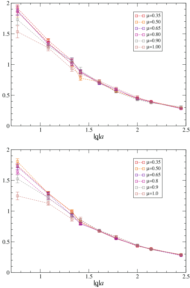
Fig. 18. As Fig. 17, for the electric gluon propagator
