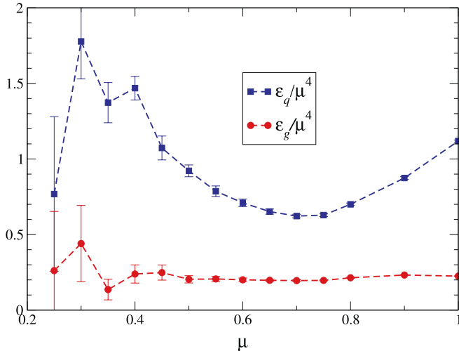
Fig. 7. Comparison of bare quark and gluon energy densities versus \mu
